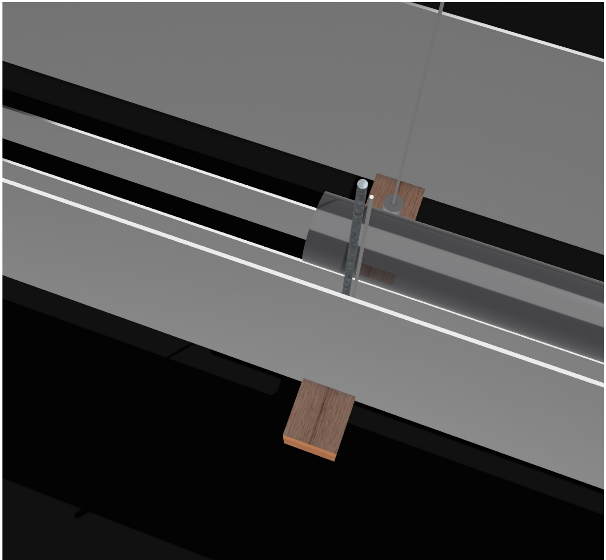
Adjustable Gallery Ceiling Hanging Sytsem with Lateral cable routing
